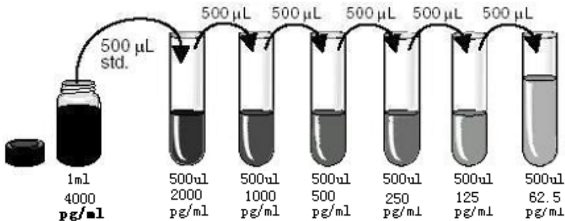
Figure 1: Preparation of MMP-9 standard dilutions
