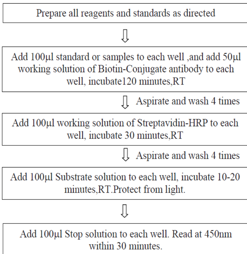
Figure 2: Assay procedure summary
