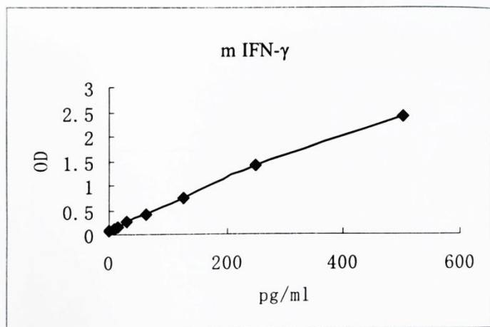
Figure 3: Representative standard curve for IFN- \gamma ELISA. IFN- \gamma was diluted in serial two-fold steps in Sample Diluent.
