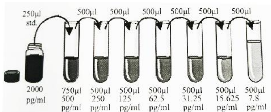
Figure 1: Preparation of IFN- \gamma standard dilutions
