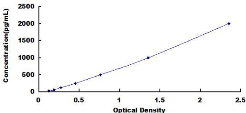
Typical Standard Curve for Mouse BNP ELISA.
