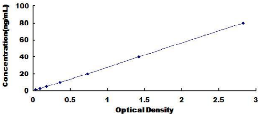
Typical Standard Curve for Rat GLUT1 ELISA.
