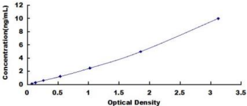
Typical Standard Curve for Human MYH9 ELISA.
