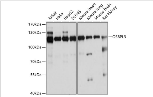
Western blot analysis of extracts of various cell lines, using OSBPL3 antibody.
