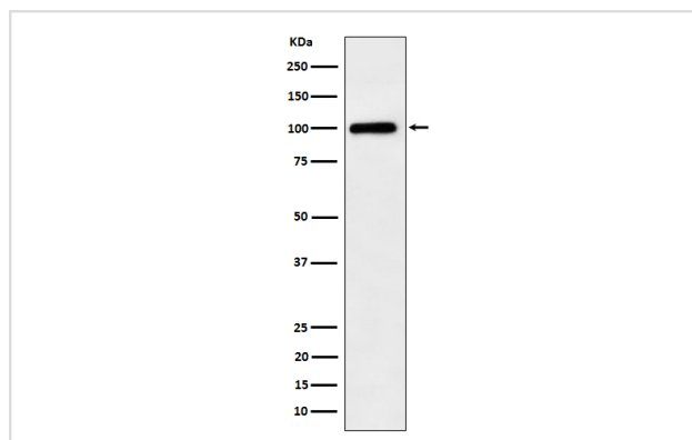
Western blot analysis of Desmocollin 1 expression in A375 cell lysate.
