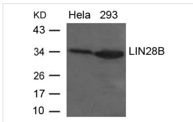
Western blot analysis of extracts from HeLa and 293 cells using LIN28B Antibody #21626.
