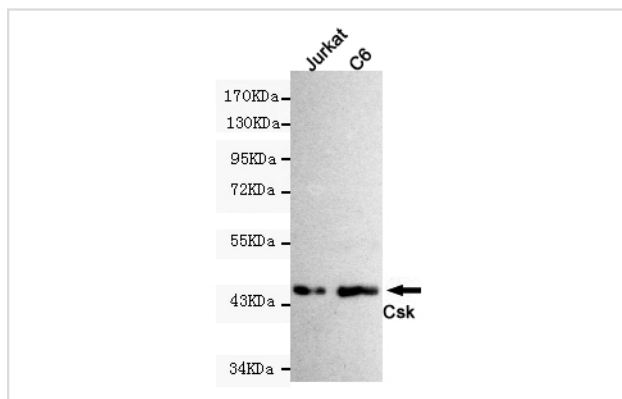
Western blot detection of CSK antibody in C6 and Jurkat cell lysates using CSK antibody (1:1000 diluted). Predicted band size: 50KDa. Observed band size: 50KDa.
