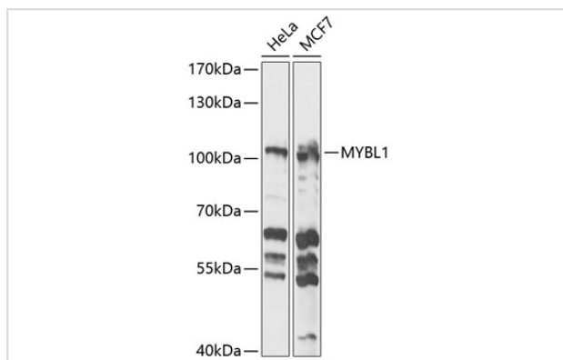
Western blot analysis of extracts of various cell lines, using MYBL1 antibody.
