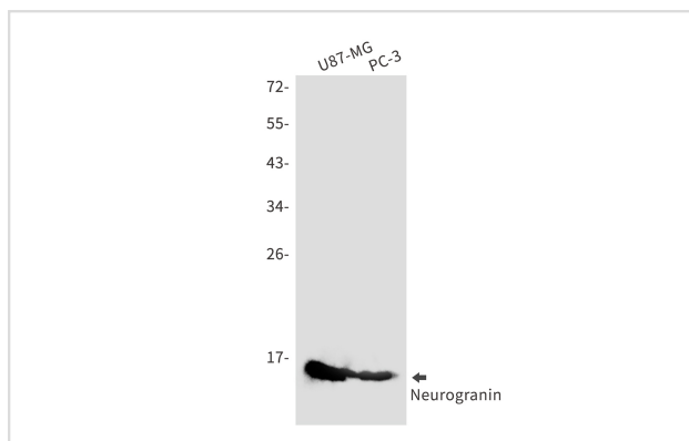
Western blot analysis of Neurogranin in U87-MG, PC-3 lysates using Neurogranin antibody.
