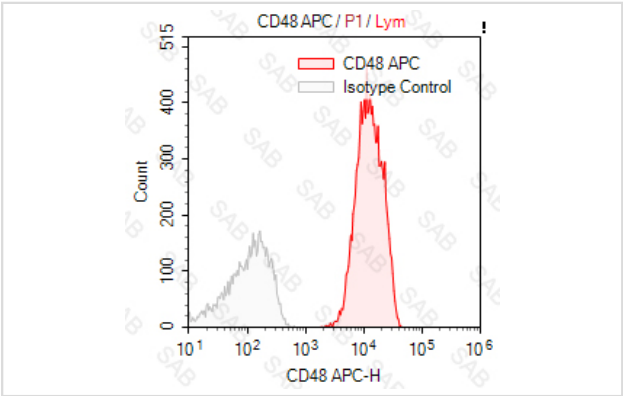
Human peripheral blood lymphocytesstained with APC anti-human CD48 (colored histogram) or APC mouse IgG1 (gray histogram)
