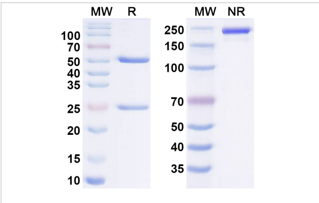
SDS-PAGE for Anti-Influenza A Virus H7 subtype Hemagglutinin/HA Antibody
