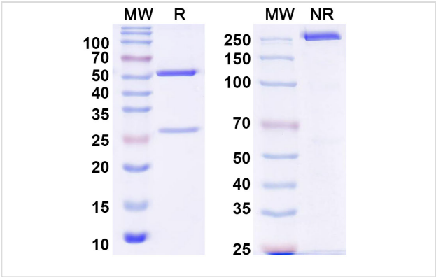
SDS-PAGE for Anti-H1N1 HA/Hemagglutinin Antibody
